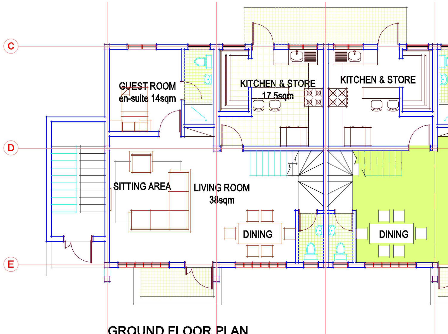
FLOOR PLAN
